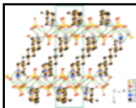
Fig. 2. The three-dimensional structure of the title compound, showing the hydrogen bonding interactions (dashed lines).
