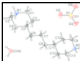
Fig. 1. A view of the title compound, showing 30% probability displacement ellipsoids.
